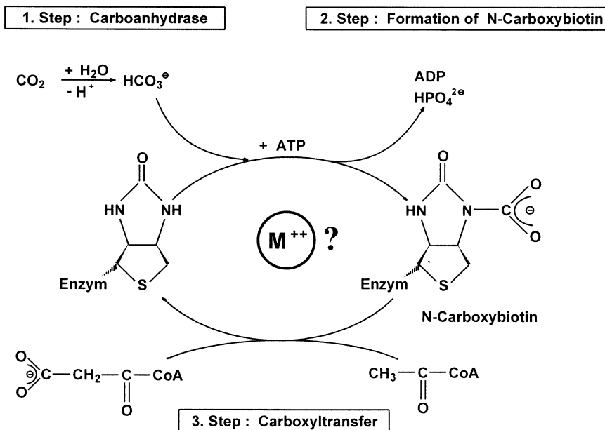
Fig. 2. Proposed catalytic cycle in biotin -depending \text{CO}_2 fixation and transfer.
