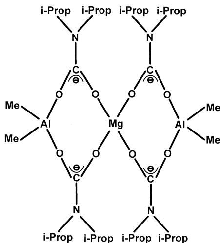
Fig. 7. Structure of a mixed Al–Mg carbamato complex [38].
