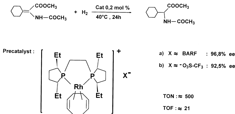
Fig. 17. Asymmetric hydrogenation of enamides in \text{scCO}_2 catalysed by Rh complexes [107].
